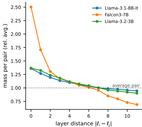
Coupling decays with layer distance
