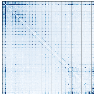
Falcon3-7B |H_{ij}| , units ordered by layer
