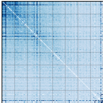
Llama-3.1-8B-It |H_{ij}| , units ordered by layer
